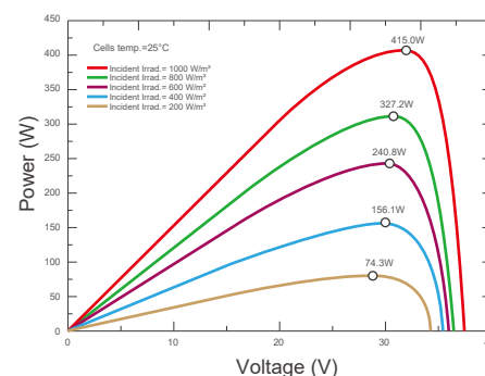
Current-Voltage & Power-Voltage Curves (RMH54-415B1)
